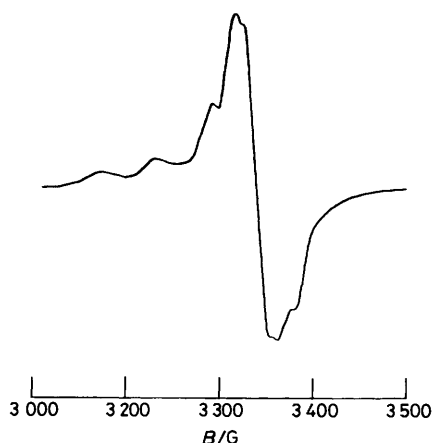
FIGURE 2 E.s.r. spectrum of \text{MoO}(\text{S}_2\text{CNET}_2)_3 in frozen toluene solution ( -140^\circ\text{C} )
