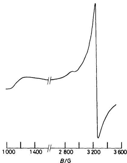
FIGURE 1 E.s.r. spectrum of a quickly frozen toluene-chloroform solution of [\text{Cr}(\text{S}_2\text{CNET}_2)_3] ( -140\text{ }^\circ\text{C} )
